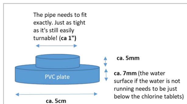
Figure 68: Plate of the Akvotur
