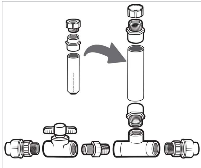
Figure 63: Assembly of the T-chlorinator parts
