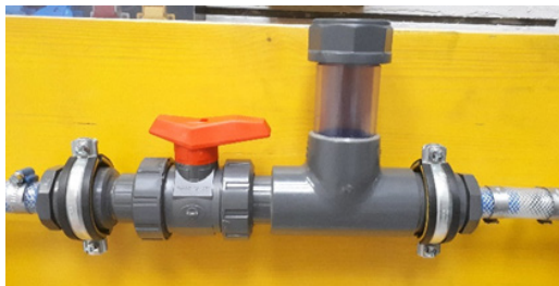
Figure 62: T-chlorinator in the laboratory at Eawag
